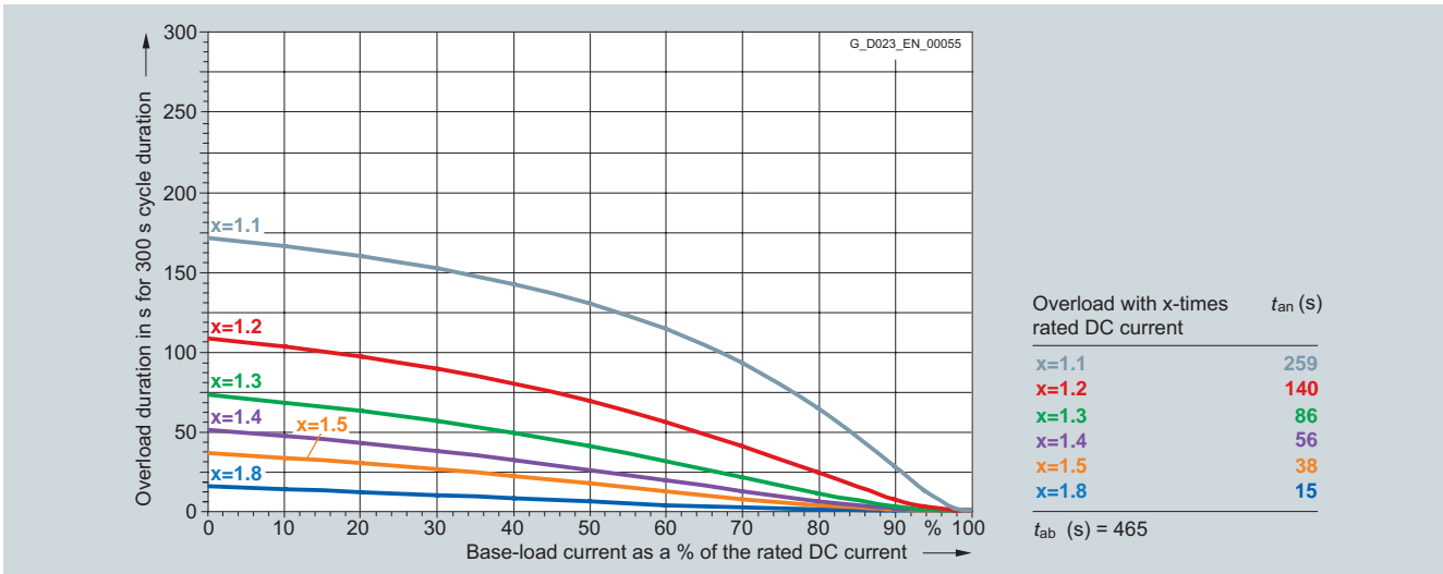
6RA8096-4MS22-0AA0 2 200 A/two-quadrant operation 950 V, 6RA8096-4MV62-0AA0 2 200 A/four-quadrant operation 950 V
