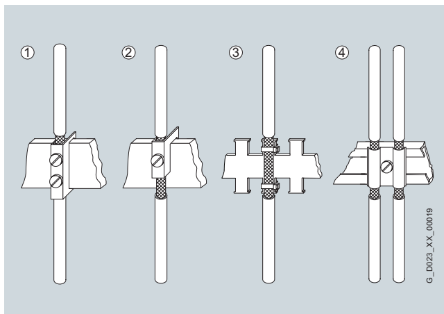
Shield connection
