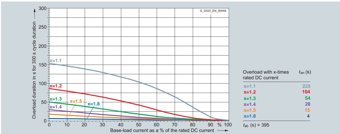
6RA8091-6DS22-0AA0 1 200 A/two-quadrant operation 400 V, 6RA8091-6FS22-0AA0 1 200 A/two-quadrant operation 480 V, 6RA8091-6FV62-0AA0 1 200 A/four-quadrant operation 480 V, 6RA8091-6DV62-0AA0 1 200 A/four-quadrant operation 400 V
