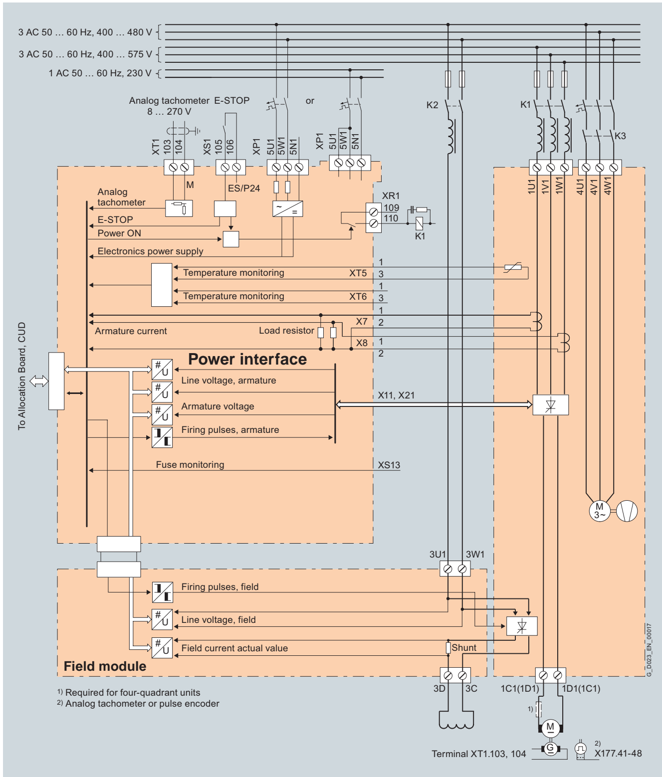
Connection diagram, DC Converters, 400 to 3 000 A, electronics power supply 400 V or 230 V, with fan
