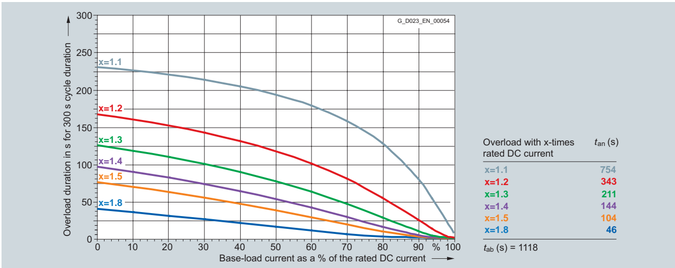
6RA8096-4GS22-0AA0 2 200 A/two-quadrant operation 575 V, 6RA8096-4GV62-0AA0 2 200 A/four-quadrant operation 575 V
