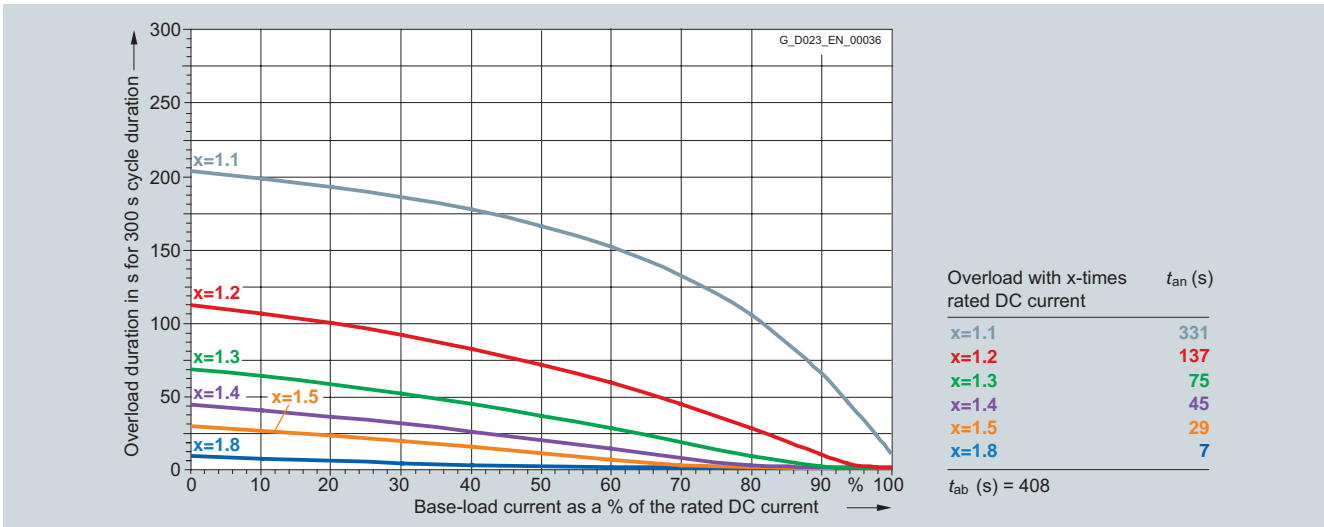
6RA8085-6DS22-0AA0 600 A/two-quadrant operation 400 V, 6RA8085-6FS22-0AA0 600 A/two-quadrant operation 480 V, 6RA8085-6GS22-0AA0 600 A/two-quadrant operation 575 V
