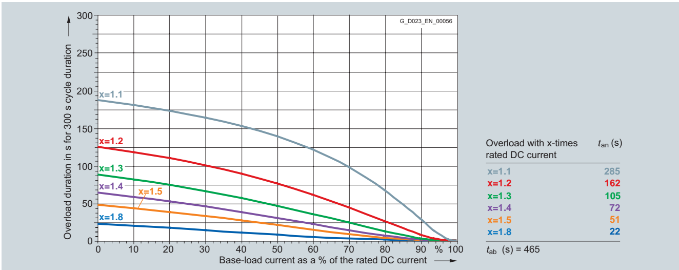
6RA8097-4GS22-0AA0 2 800 A/two-quadrant operation 575 V, 6RA8097-4GV62-0AA0 2 800 A/four-quadrant operation 575 V
