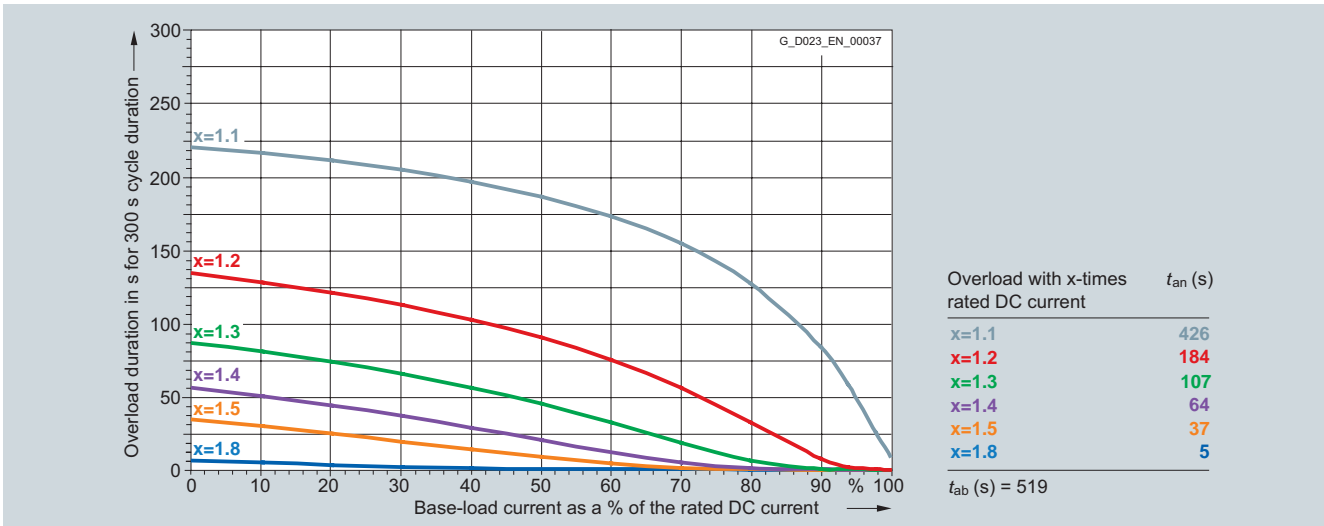
6RA8085-6DV62-0AA0 600 A/four-quadrant operation 400 V, 6RA8085-6FV62-0AA0 600 A/four-quadrant operation 480 V, 6RA8085-6GV62-0AA0 600 A/four-quadrant operation 575 V
