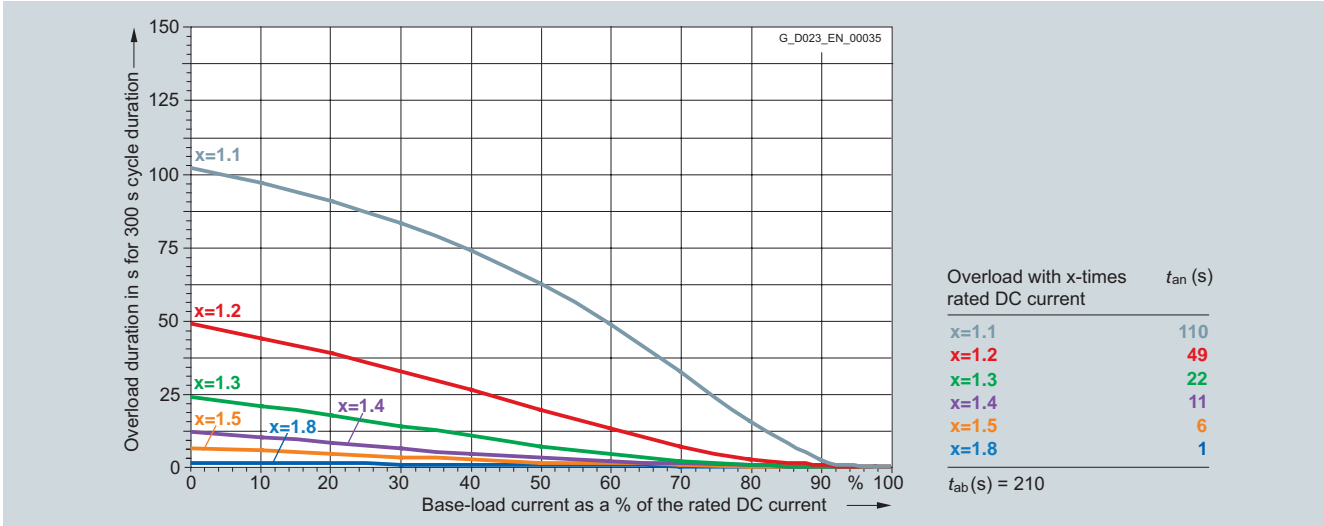
6RA8082-6FS22-0AA0 450 A/two-quadrant operation 480 V, 6RA8082-6FV62-0AA0 450 A/four-quadrant operation 480 V
